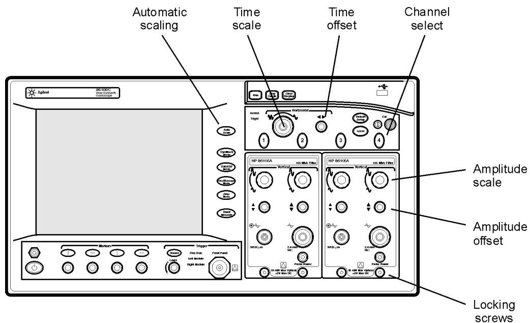
Figure 2-6. Amplitude and time adjustments
