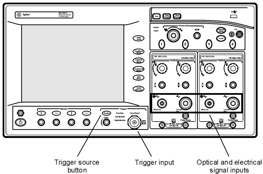
Figure 2-3. Trigger Controls
