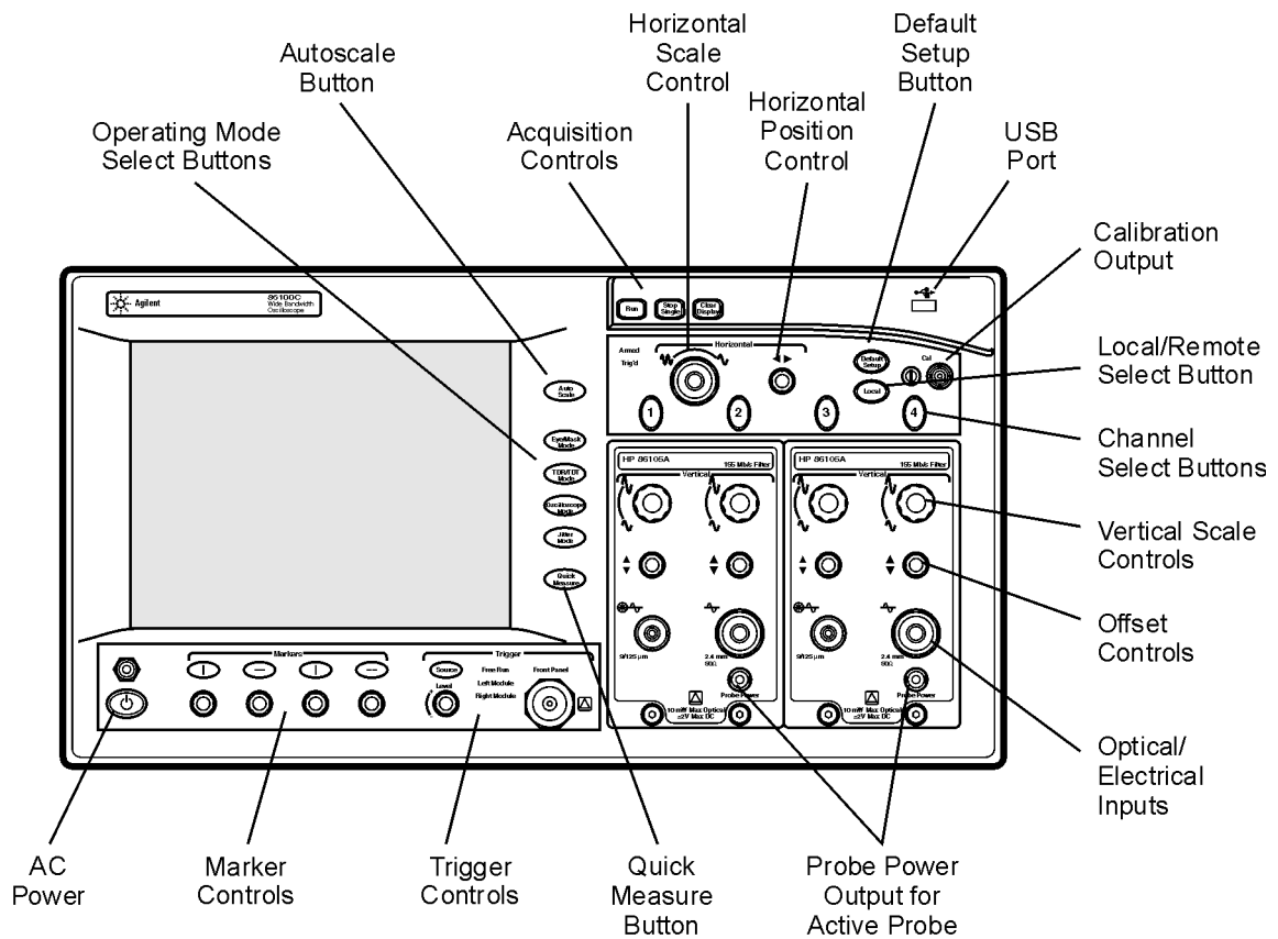
Figure 2-4. Front-Panel Features
