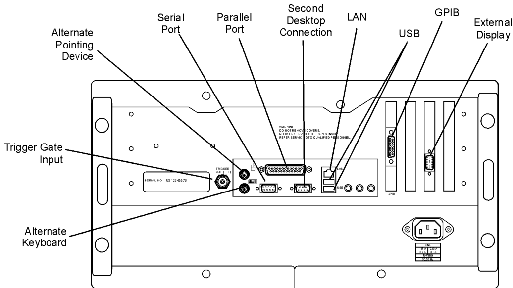
Figure 2-5. Rear-Panel Features
