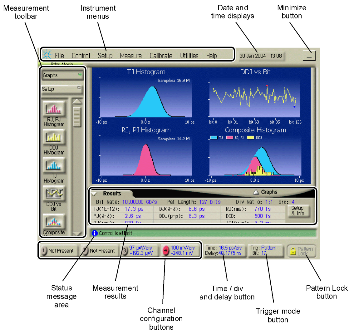
Figure 2-2. Display
