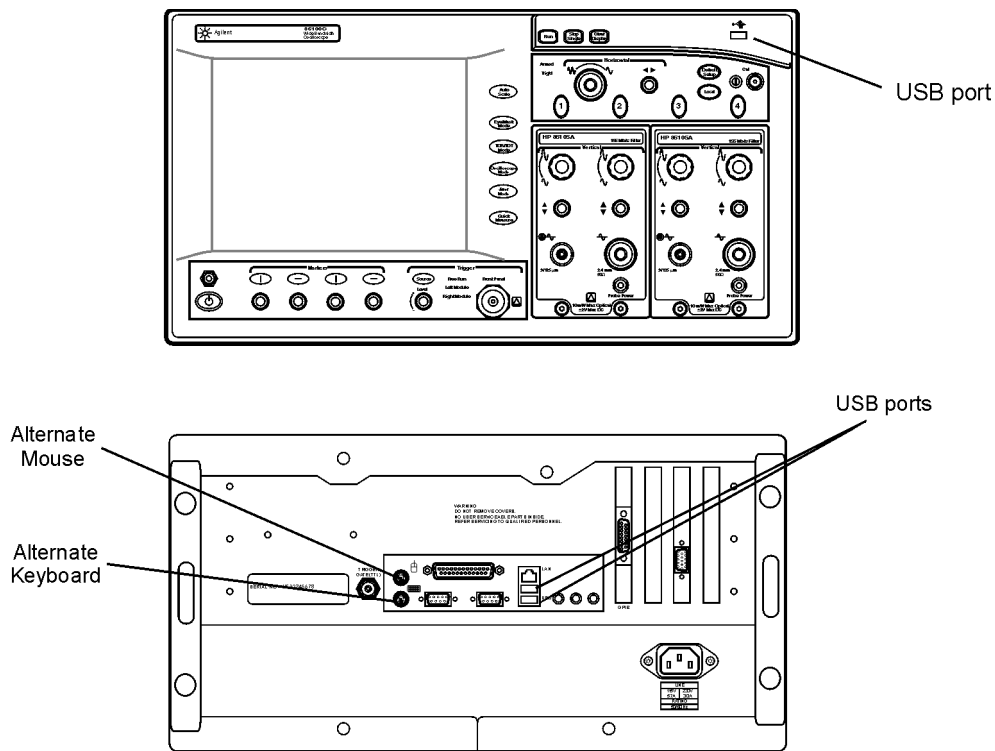
Figure 1-3. Accessory Connections
